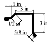
ORG9 9 5/8"
