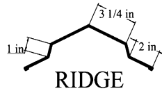
ORR1 13 1/2" T
