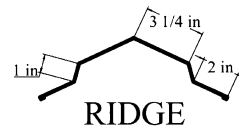
ORR1 13 1/2" T
