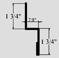
ZEE TRIM
