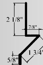
BASE GUARD
