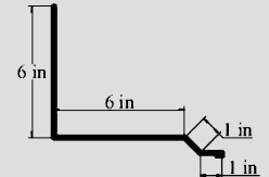
SIDEWALL
