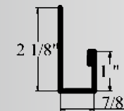
J TRIM
