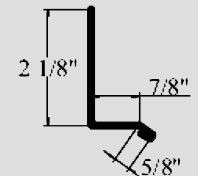
DRIP CAP
